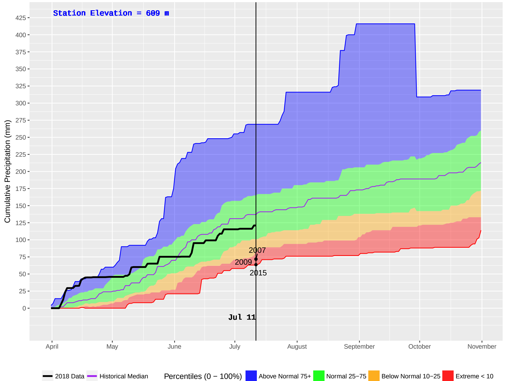
ROCK CREEK (394) : Historical (1990–2016) and Current (2018) Noon Cumulative Precipitation
